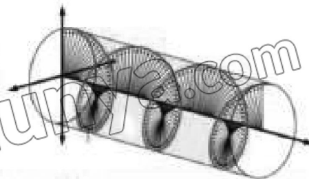
Fig. 8.4 (b): Circular polarization of light
