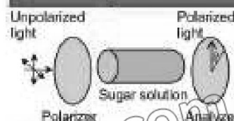
Fig. 8.8: Optical activity
