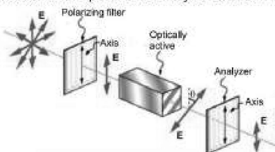
Fig. 8.8: Optical activity
