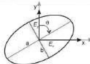
Fig. 8.4 (c): Elliptical polarization of light
