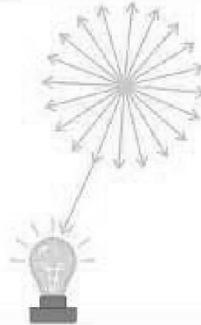
Fig. 8.2: An unpolarized light, due to incandescent bulb, has vibrations in all directions.
