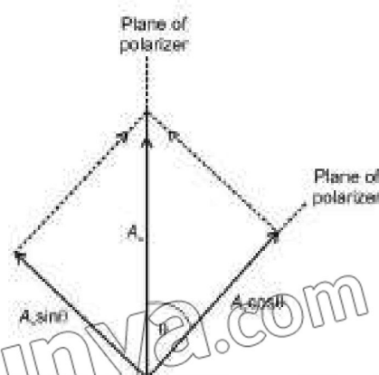
Fig. 8.7(b): Resolution of amplitude into components of plane polarization light.
