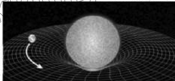
Spacetime curve shown by two satellites
