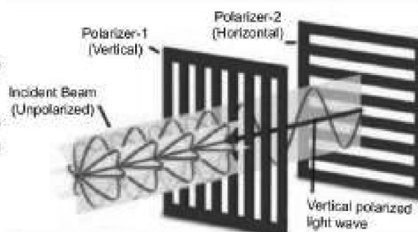
Light passing through crossed polarizers
