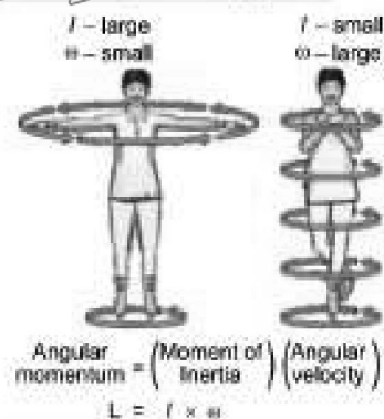
Fig. 3.19 An ice skater using angular momentum
