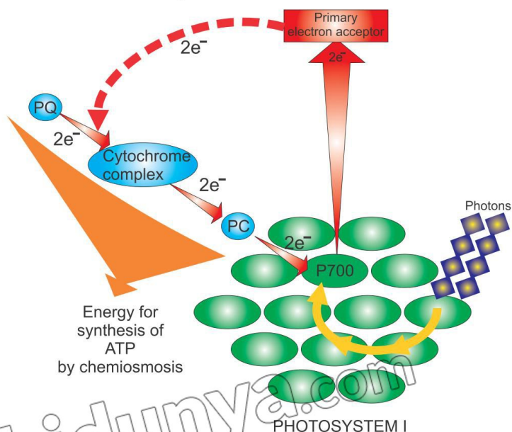
Figure 5.10: Cyclic Photophosphorylation
