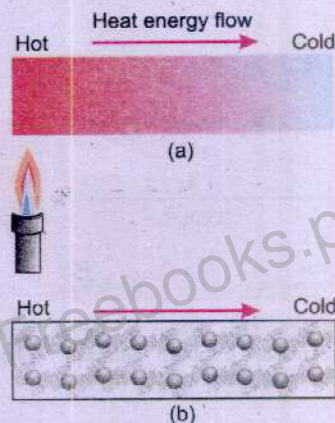
Figure 9.2: In solids, heat is transferred from one part to other parts from atoms to atoms or
