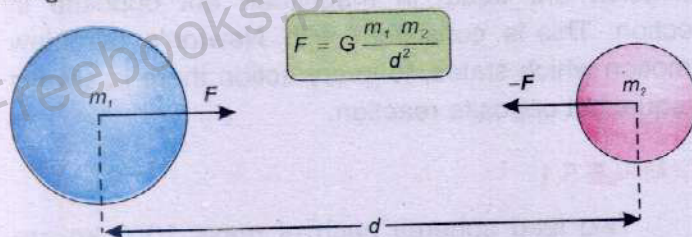
Figure 5.1: Two masses attract each other with a gravitational force of
