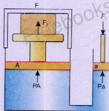
Figure 7.16: A hydraulic press
