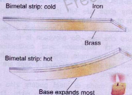
Figure 8.19 (a) A bimetal strip of brass and iron (b) Bending of brass-iron bimetal strip on heating due to the difference in their thermal expansion.
