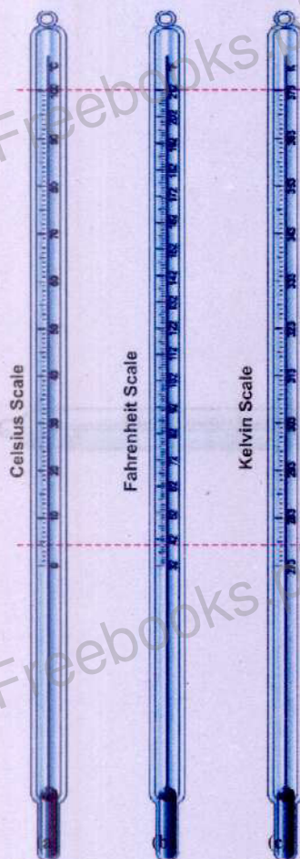
Figure 8.5: Various scales of temperature.
