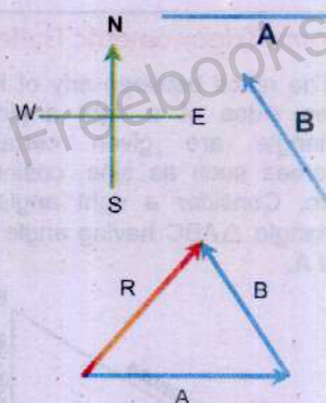
Figure 4.5: Adding vectors by head to tail rule.
